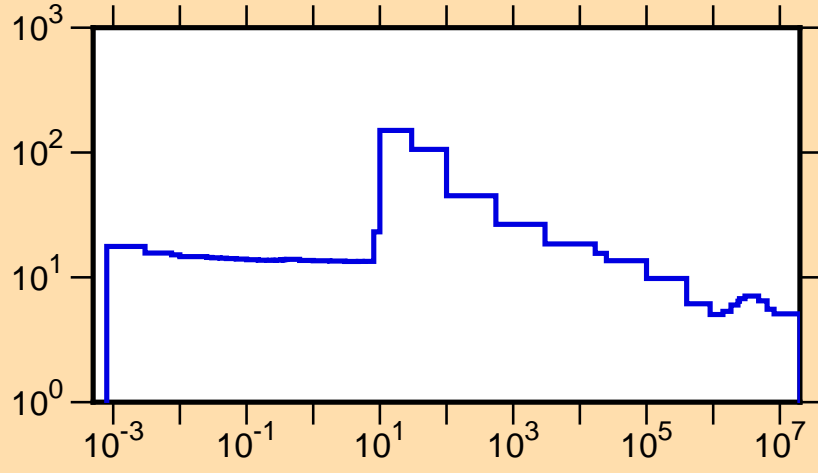
\sigma vs. E for ^{194}\text{Tl}(n,\text{tot.})
