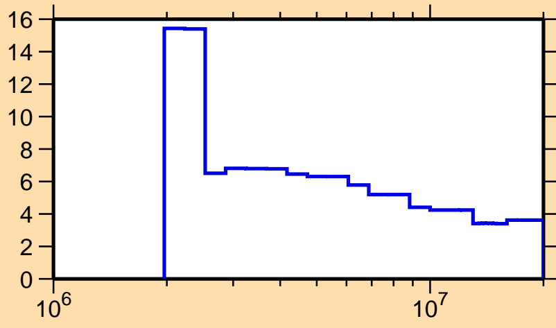
\Delta\sigma/\sigma vs. E for ^{195}\text{Tl}(n, n\text{onel.})
