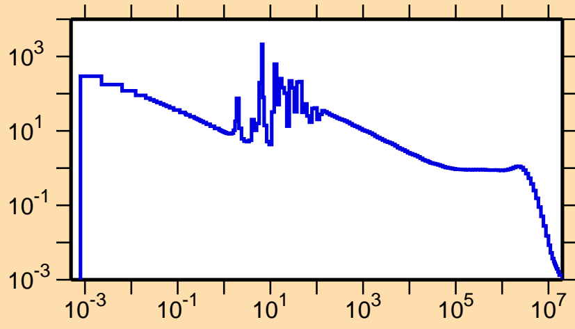
\sigma vs. E for ^{195}\text{Tl}(n,\gamma)
