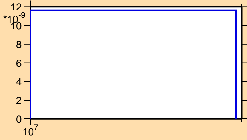
\sigma vs. E for ^{195}\text{Tl}(n,\text{nd})
