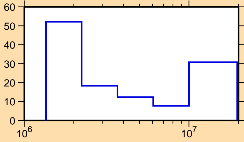
\Delta\sigma/\sigma vs. E for ^{195}\text{Tl}(n,ncont.)
