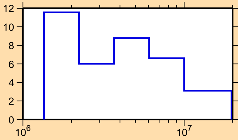
\Delta\sigma/\sigma vs. E for ^{195}\text{Tl}(n,\text{tot.})
