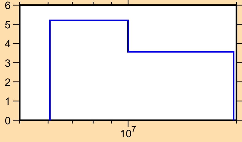
\Delta\sigma/\sigma vs. E for ^{195}\text{Tl}(n,\text{nonel.})
