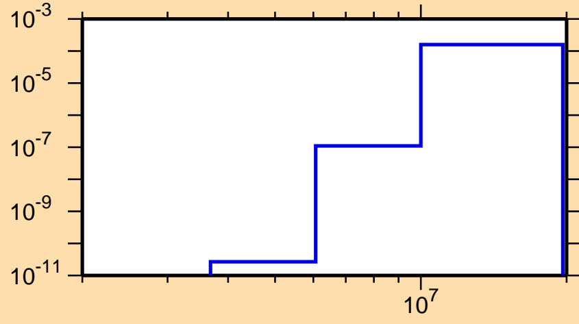
\sigma vs. E for ^{195}\text{Tl}(n,n\alpha)
