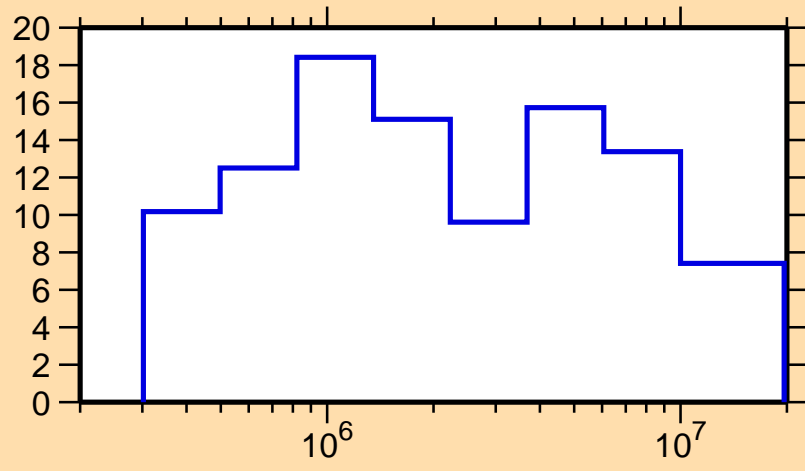
\Delta\sigma/\sigma vs. E for ^{195}\text{Tl}(n,\text{el.})
