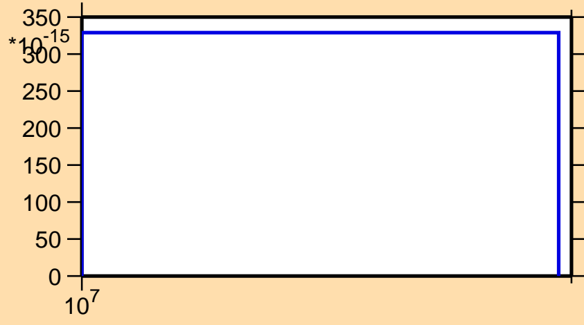
\sigma vs. E for ^{195}\text{Tl} (mt 45)
