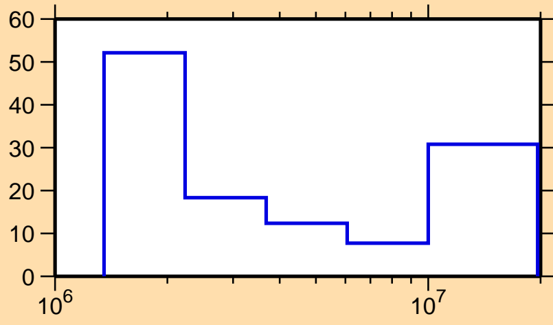
\Delta\sigma/\sigma vs. E for ^{195}\text{Tl}(n,n\text{cont.})
