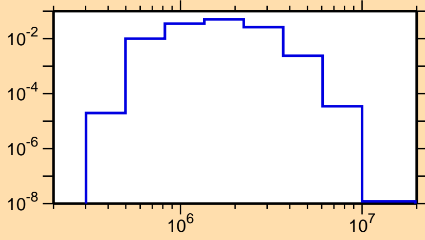
\sigma vs. E for ^{195}\text{Tl}(n,n_2)
