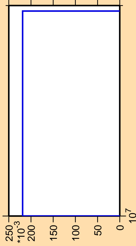
\Delta\sigma/\sigma vs. E for ^{195}\text{Tl}(\text{mt117})
