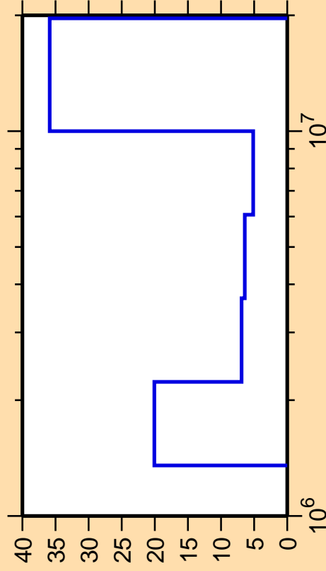
\Delta\sigma/\sigma vs. E for ^{195}\text{Tl}(n,n\text{cont.})
