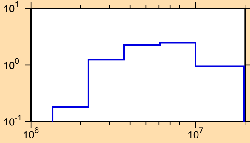
\sigma vs. E for ^{195}\text{Tl}(n,n\text{cont.})
