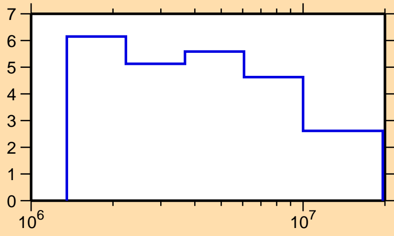
\Delta\sigma/\sigma vs. E for ^{195}\text{Tl}(n, \text{tot.})
