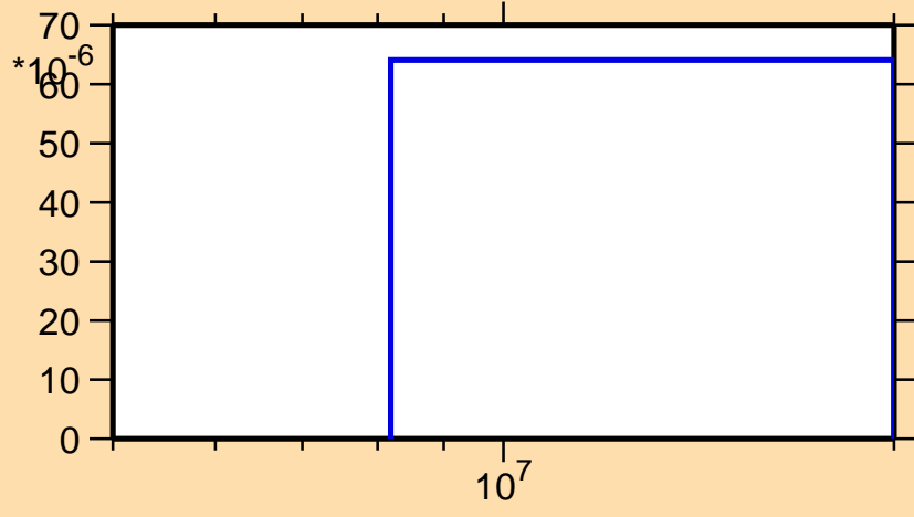
\sigma vs. E for ^{195}\text{Tl}(n,t)
