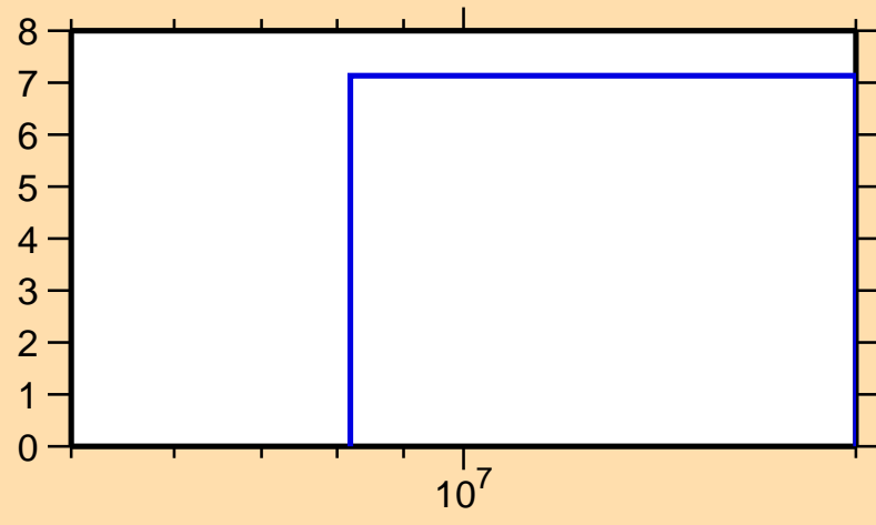
\Delta\sigma/\sigma vs. E for ^{195}\text{Tl}(n,\text{el.})
