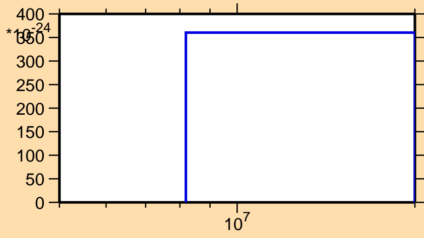
\sigma vs. E for ^{195}\text{Tl} (mt 42)
