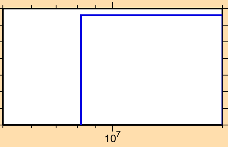
\sigma vs. E for ^{195}\text{Tl}(n,3n)
