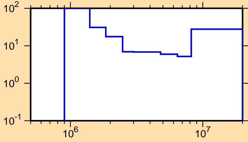
\Delta\sigma/\sigma vs. E for ^{195}\text{Tl}(n,n\text{cont.})
