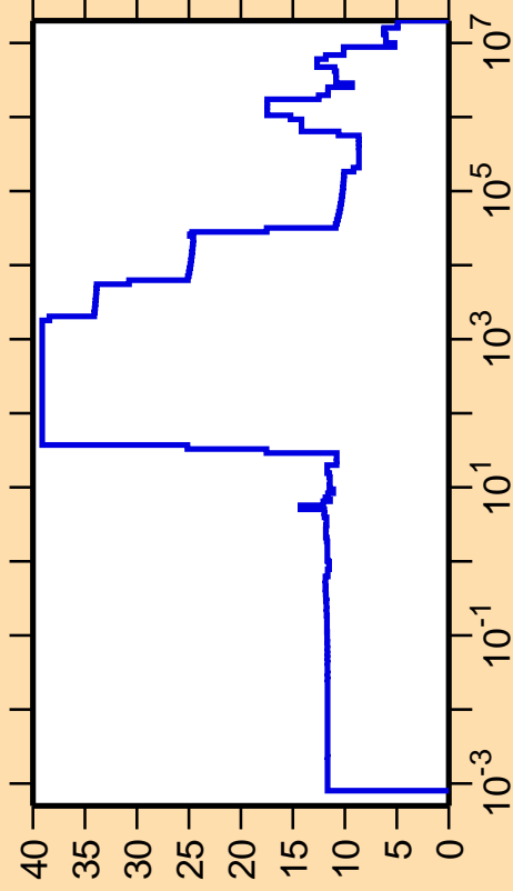
\Delta\sigma/\sigma vs. E for ^{196}\text{Tl}(n,\text{el.})
