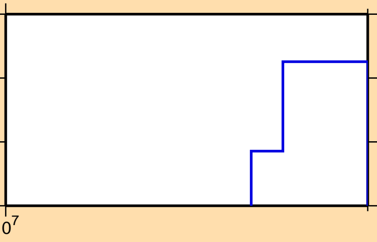
\sigma vs. E for ^{196}\text{Tl} (mt 45)
