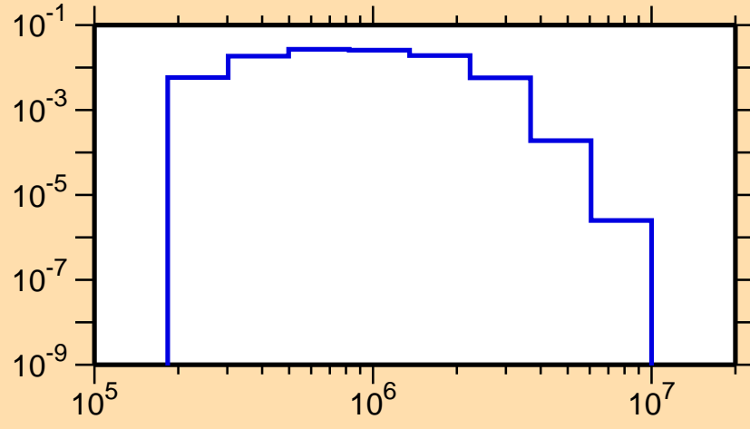
\sigma vs. E for ^{196}\text{Tl}(n,n_1)
