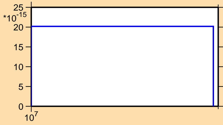
\sigma vs. E for ^{196}\text{Tl} (mt 45)
