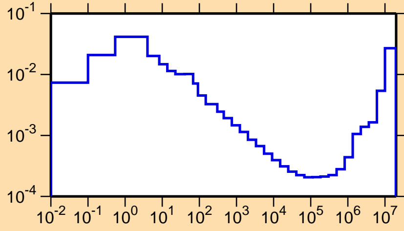
\sigma vs. E for ^{196}\text{Tl}(n,p)
