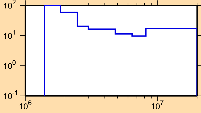
\Delta\sigma/\sigma vs. E for ^{196}\text{Tl}(n,n\text{cont.})
