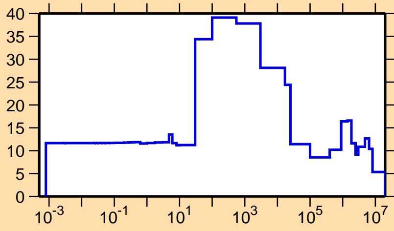
\Delta\sigma/\sigma vs. E for ^{196}\text{Tl}(n,el.)
