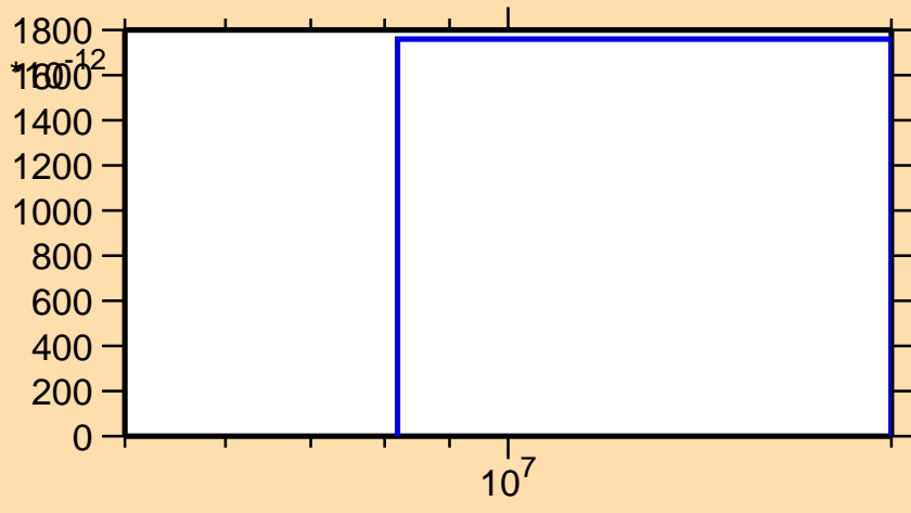
\sigma vs. E for ^{196}\text{Tl}(n,p\alpha)
