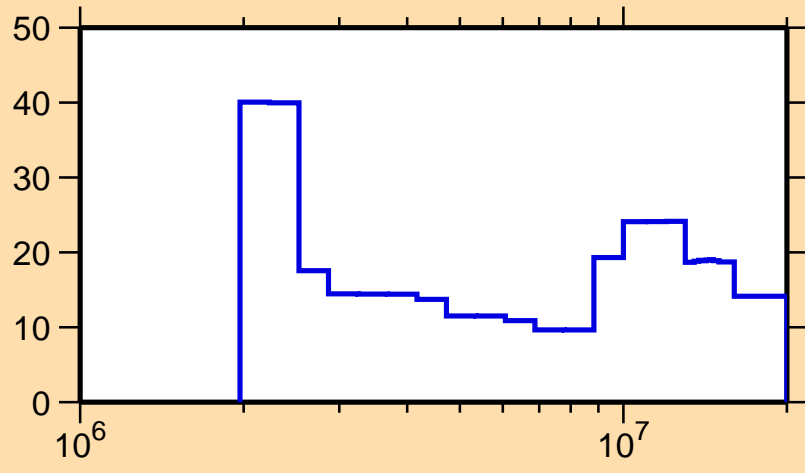
\Delta\sigma/\sigma vs. E for ^{197}\text{Tl}(n,ncont.)
