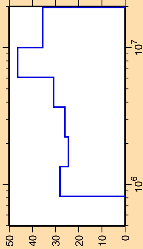
\Delta\sigma/\sigma vs. E for ^{197}\text{Tl}(n,n_4)
