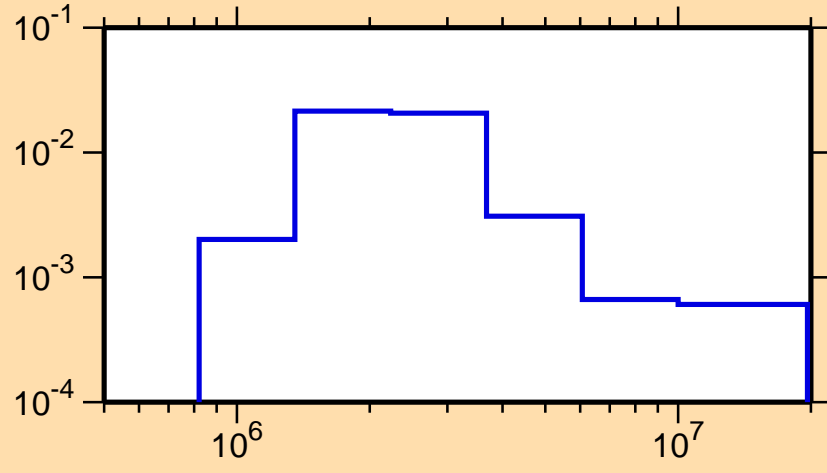
\sigma vs. E for ^{197}\text{Tl}(n,n_4)
