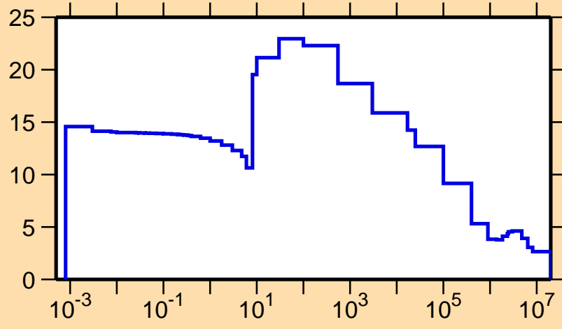
\sigma vs. E for ^{197}\text{Tl}(n,\text{el.})
