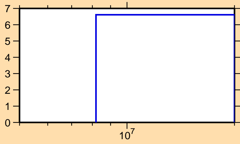
\Delta\sigma/\sigma vs. E for ^{197}\text{Tl}(n,\text{nonel.})
