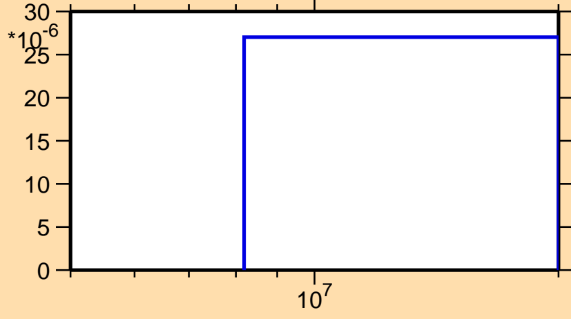
\sigma vs. E for ^{197}\text{Tl}(n,t)
