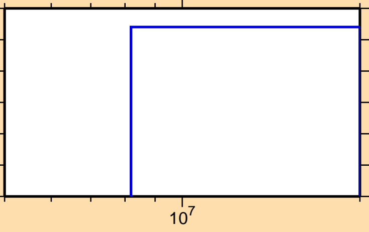
\sigma vs. E for ^{197}\text{Tl}(n,t)
