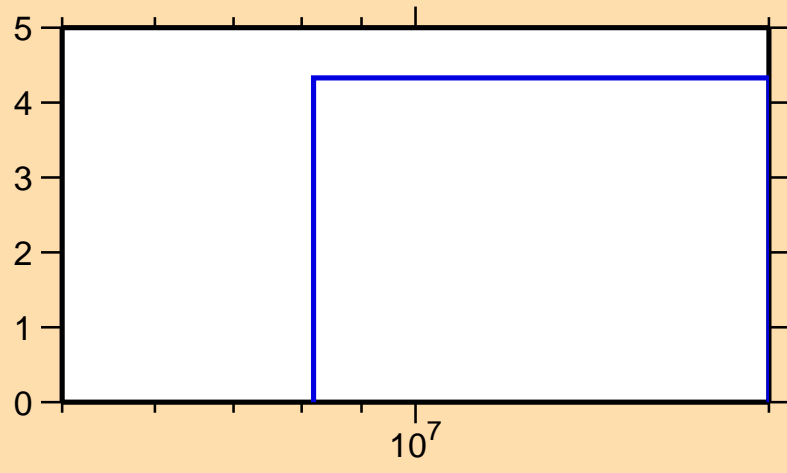
\Delta\sigma/\sigma vs. E for ^{197}\text{Tl}(n,\text{el.})
