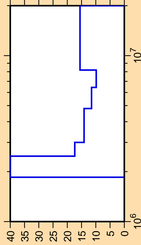
\Delta\sigma/\sigma vs. E for ^{197}\text{Tl}(n,n\text{cont.})
