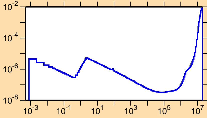
\sigma vs. E for ^{198}\text{Tl}(n,\alpha)
