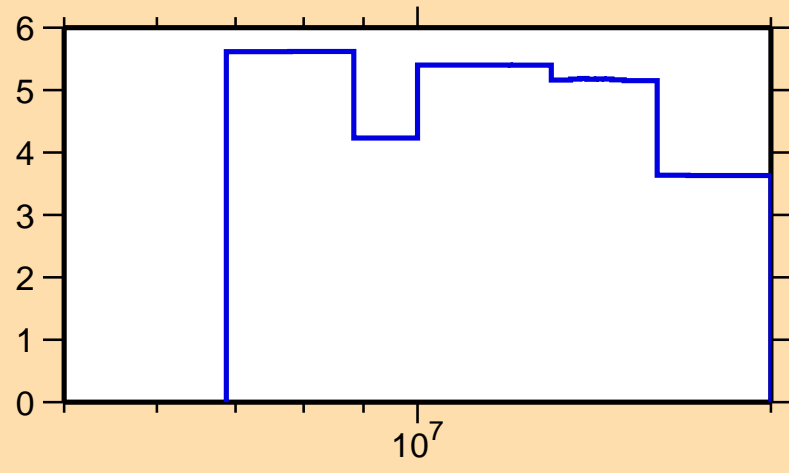
\Delta\sigma/\sigma vs. E for ^{198}\text{Tl}(n,\text{el.})
