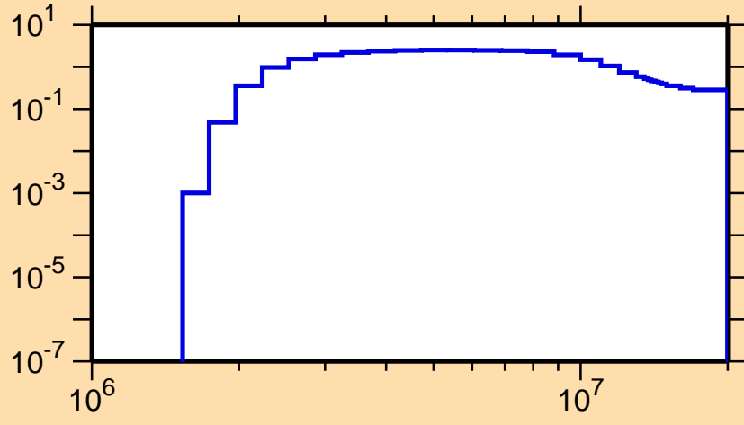
\sigma vs. E for ^{198}\text{Tl}(n,n\text{cont.})
