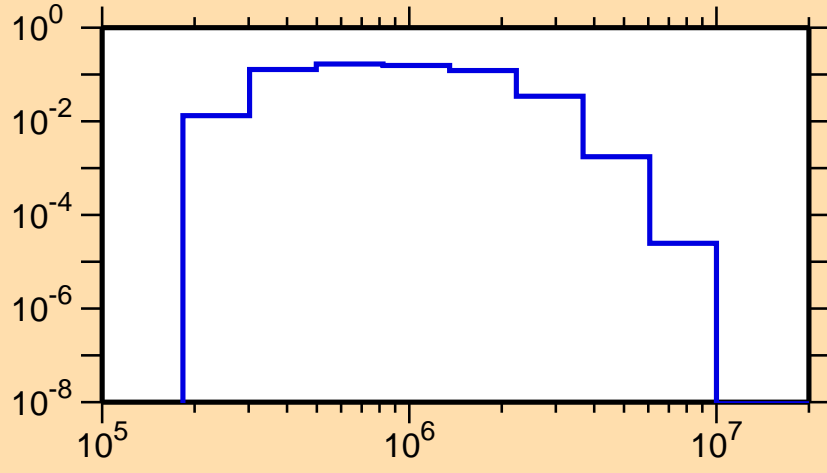
\sigma vs. E for ^{198}\text{Tl}(n,n_2)
