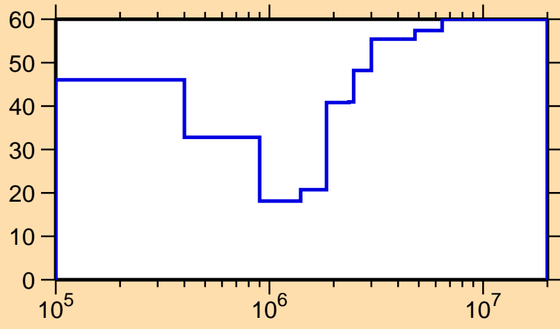
\Delta\sigma/\sigma vs. E for ^{198}\text{Tl}(n,n_1)
