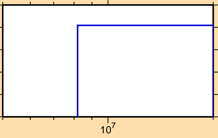
\sigma vs. E for ^{198}\text{Tl}(n,2np)
