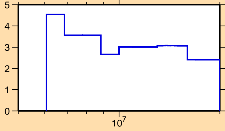
\Delta\sigma/\sigma vs. E for ^{198}\text{Tl}(n,\text{tot.})
