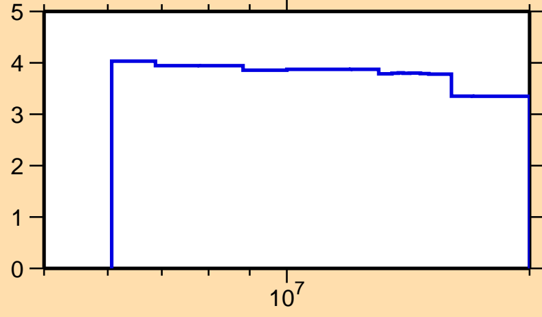
\Delta\sigma/\sigma vs. E for ^{198}\text{Tl}(n,\text{nonel.})
