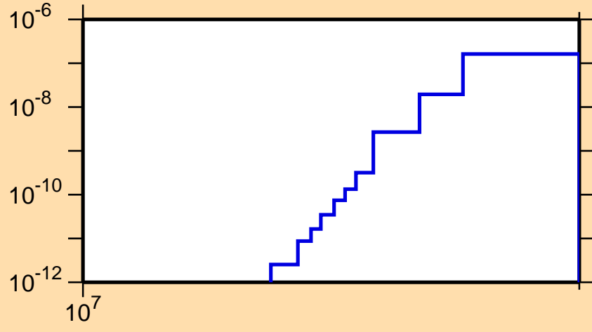
\sigma vs. E for ^{198}\text{Tl}(n,2n\alpha)
