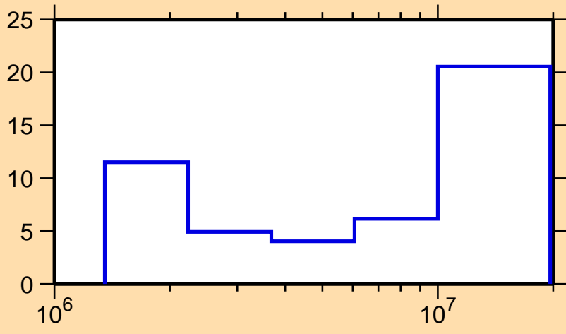
\Delta\sigma/\sigma vs. E for ^{198}\text{Tl}(n,n\text{cont.})
