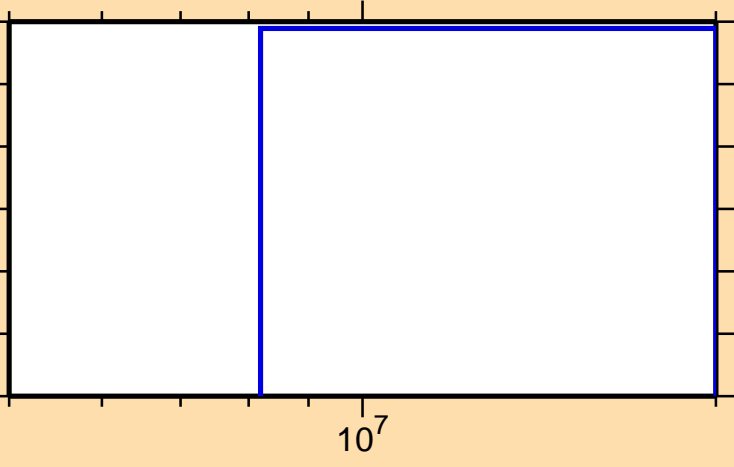
\sigma vs. E for ^{198}\text{Tl}(\text{mt } 34)
