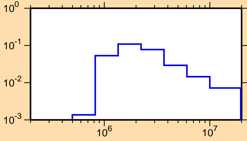
\sigma vs. E for ^{199}\text{Tl}(n,n_3)
