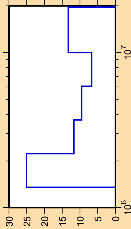
\Delta\sigma/\sigma vs. E for ^{199}\text{Tl}(n,n\text{cont.})
