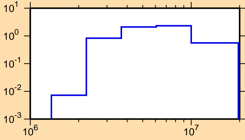
\sigma vs. E for ^{199}\text{Tl}(n,n\text{cont.})
