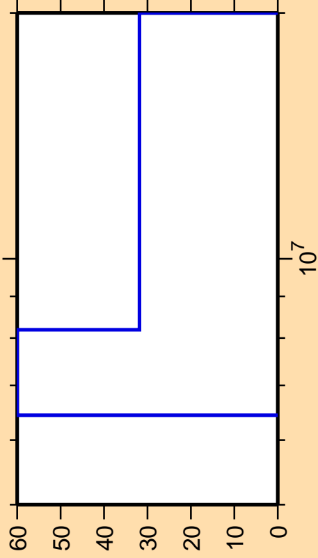
\Delta\sigma/\sigma vs. E for ^{199}\text{Tl}(n,np)
