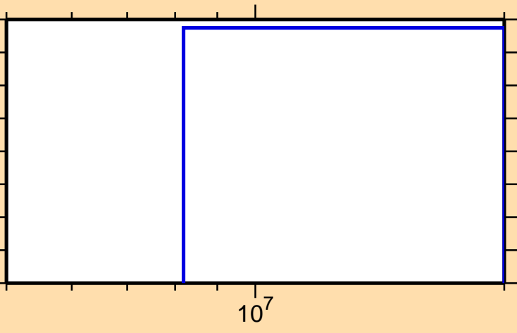
\sigma vs. E for ^{199}\text{Tl}(n,3n)
