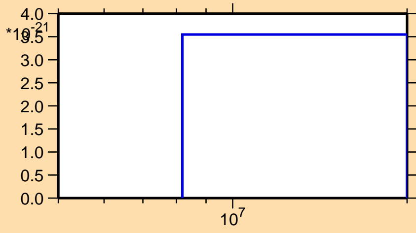
\sigma vs. E for ^{199}\text{Tl} (mt 42)
