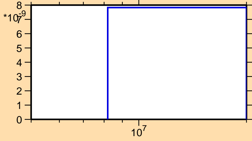
\sigma vs. E for ^{199}\text{Tl}(n,\text{nd})
