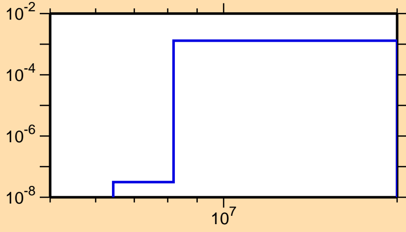
\sigma vs. E for ^{199}\text{Tl}(n,np)
