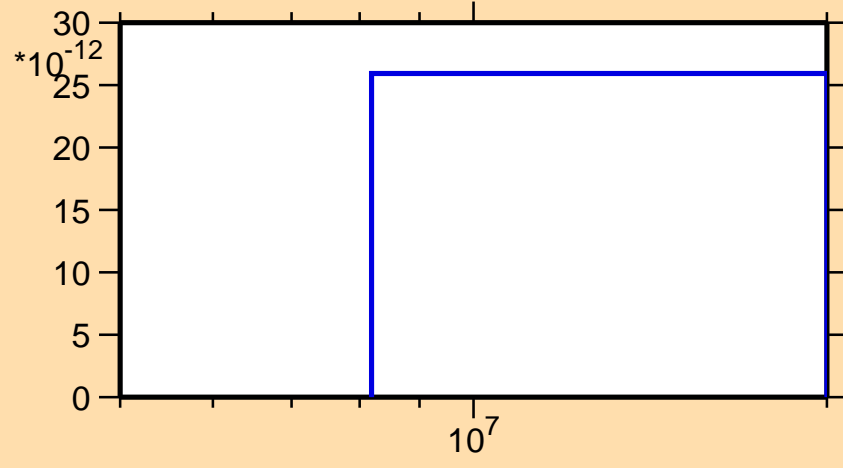
\sigma vs. E for ^{199}\text{Tl}(n,2n\alpha)
