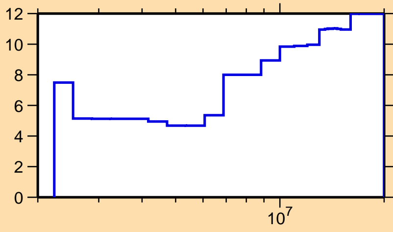
\Delta\sigma/\sigma vs. E for ^{200}\text{Tl}(n,ncont.)
