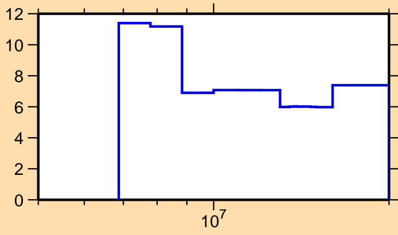
\Delta\sigma/\sigma vs. E for ^{200}\text{Tl}(n,2n)
