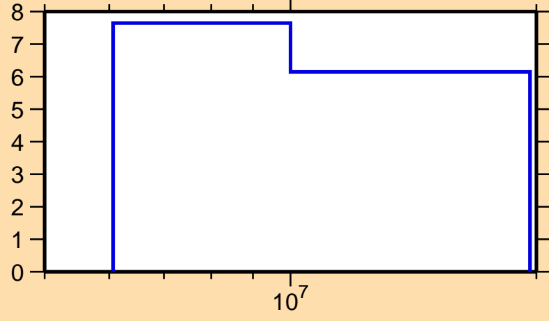
\Delta\sigma/\sigma vs. E for ^{200}\text{Tl}(n,2n)
