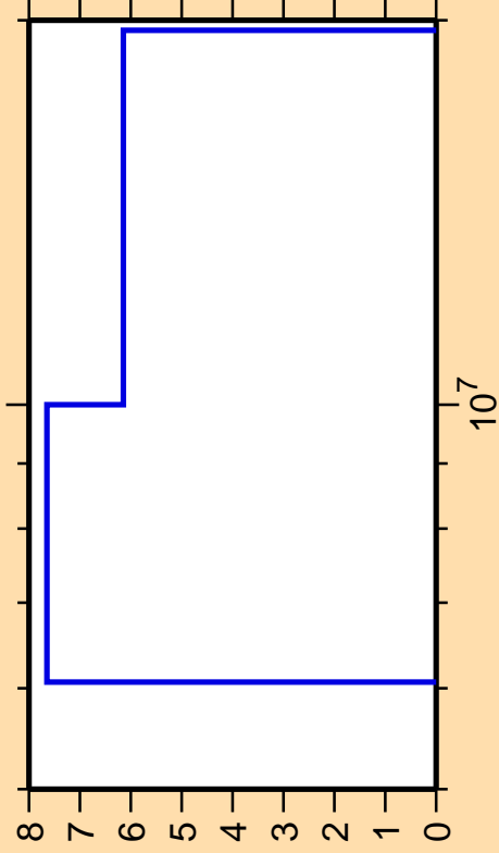
\Delta\sigma/\sigma vs. E for ^{200}\text{Tl}(n,2n)
