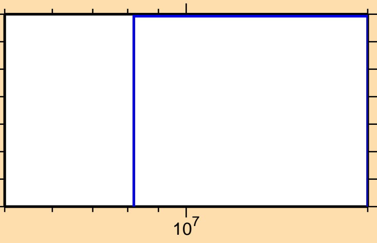
\sigma vs. E for ^{200}\text{Tl}(n,p\alpha)
