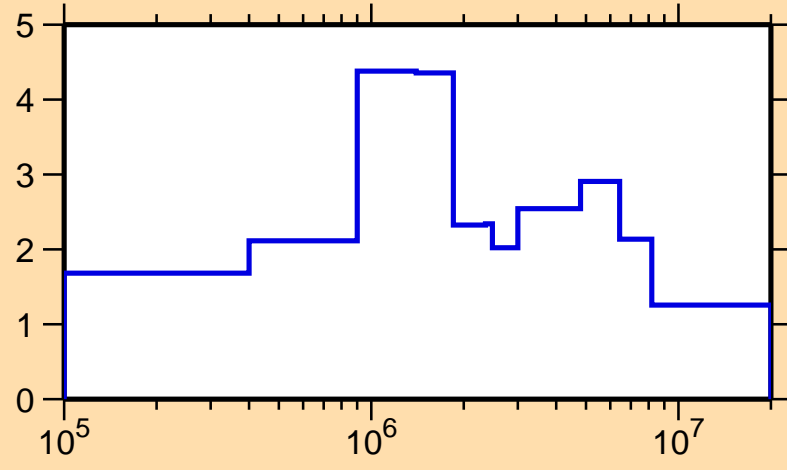
\Delta\sigma/\sigma vs. E for ^{200}\text{Tl}(n,\text{el.})
