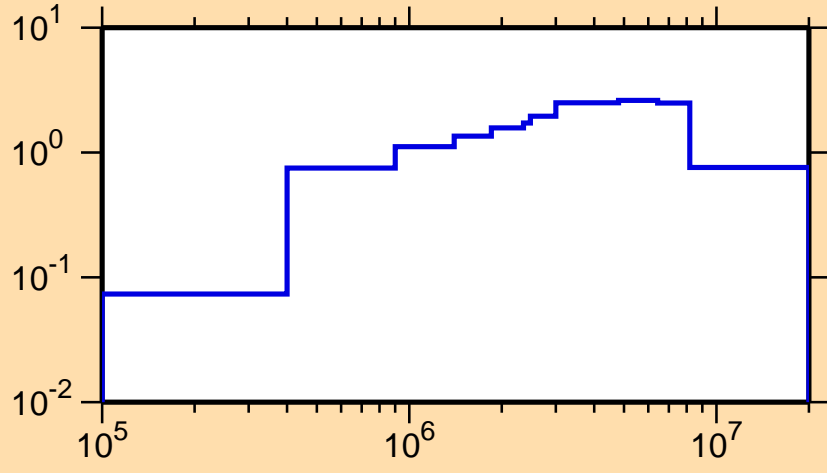
\sigma vs. E for ^{200}\text{Tl}(n,\text{inel.})
