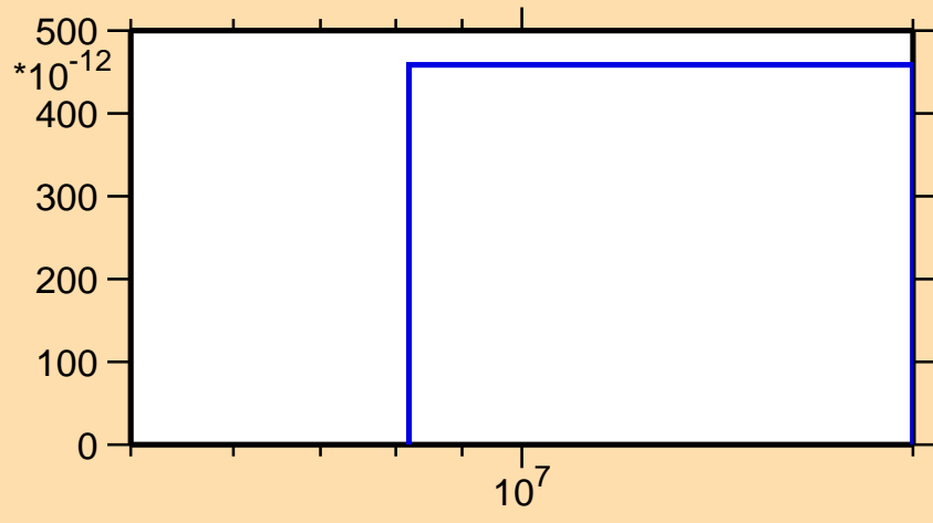
\sigma vs. E for ^{200}\text{Tl}(n,nt)
