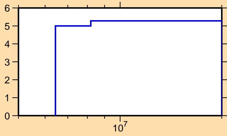
\Delta\sigma/\sigma vs. E for ^{200}\text{Tl}(n,\text{nonel.})
