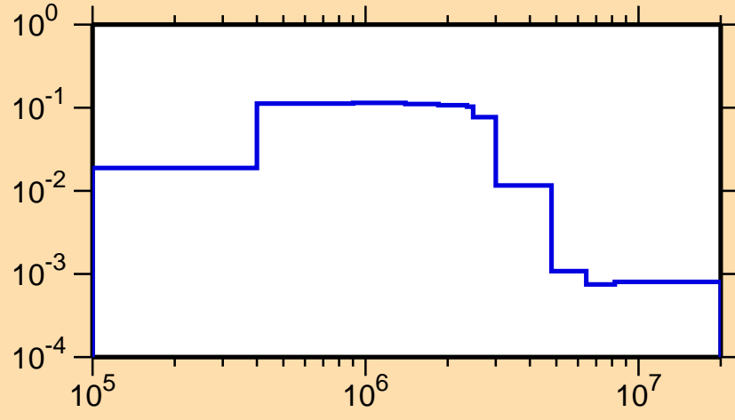
\sigma vs. E for ^{200}\text{Tl}(n,n_2)
