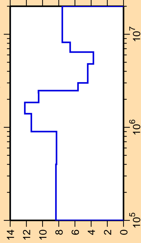
\Delta\sigma/\sigma vs. E for ^{200}\text{Tl}(n,\text{inel.})
