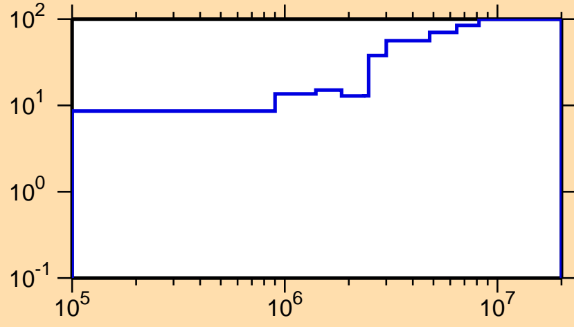
\Delta\sigma/\sigma vs. E for ^{200}\text{Tl}(n,n_1)
