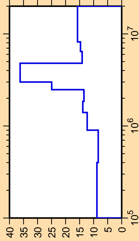
\Delta\sigma/\sigma vs. E for ^{200}\text{Tl}(n,n_4)
