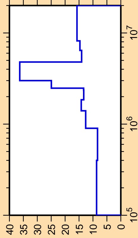
\Delta\sigma/\sigma vs. E for ^{200}\text{Tl}(n,n_2)
