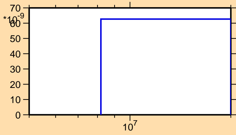
\sigma vs. E for ^{200}\text{Tl}(n,nd)
