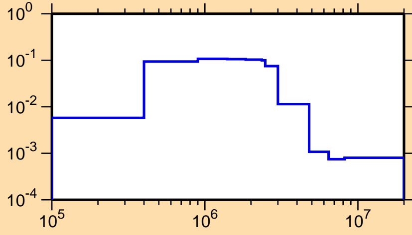
\sigma vs. E for ^{200}\text{Tl}(n,n_4)
