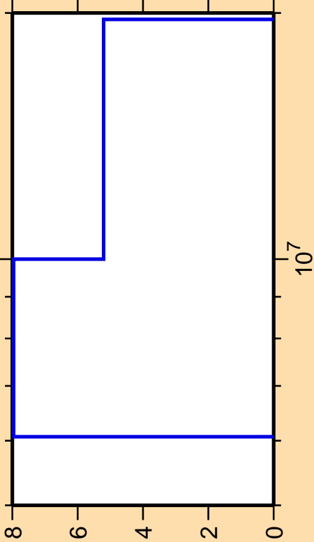
\Delta\sigma/\sigma vs. E for ^{201}\text{Tl}(n,2n)
