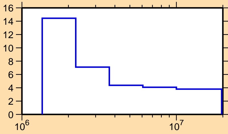
\Delta\sigma/\sigma vs. E for ^{201}\text{Tl}(n,n\text{onel.})
