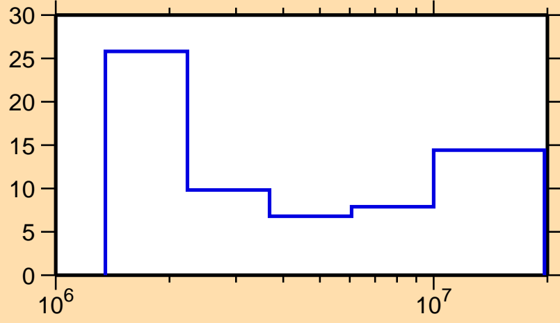
\Delta\sigma/\sigma vs. E for ^{201}\text{Tl}(n,n\text{cont.})
