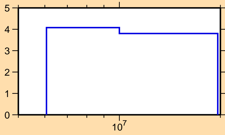
\Delta\sigma/\sigma vs. E for ^{201}\text{Tl}(n,\text{nonel.})
