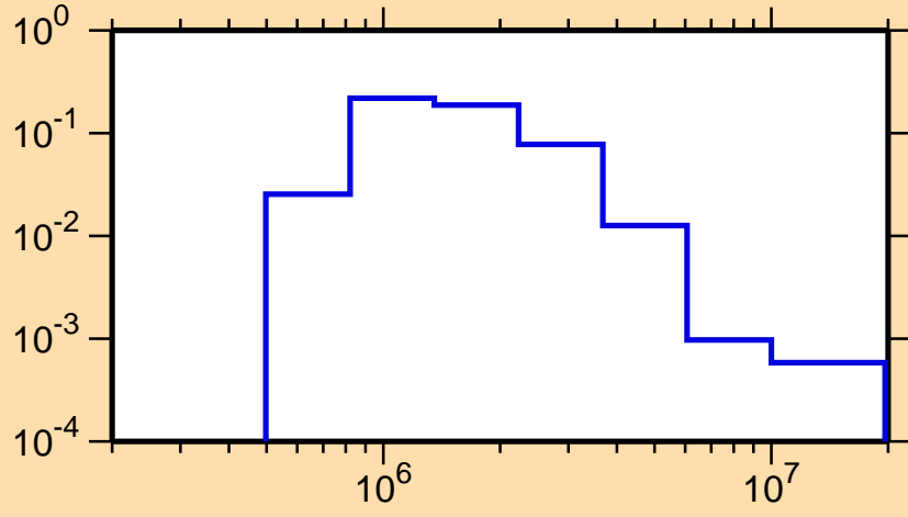
\sigma vs. E for ^{201}\text{Tl}(n,n_2)
