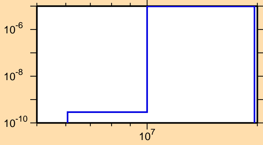
\sigma vs. E for ^{201}\text{Tl}(n,n\alpha)
