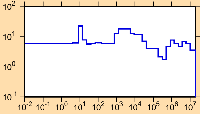
\Delta\sigma/\sigma vs. E for ^{202}\text{Tl}(n,el.)
