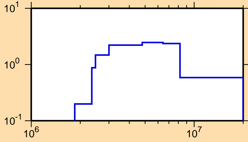
\sigma vs. E for ^{202}\text{Tl}(n,n\text{cont.})
