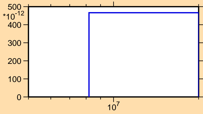
\sigma vs. E for ^{202}\text{Tl}(n,nt)
