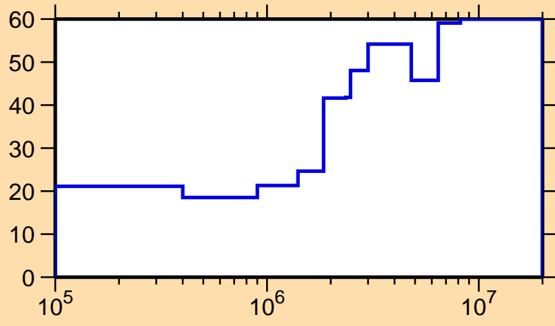
\Delta\sigma/\sigma vs. E for ^{202}\text{Tl}(n,n_1)
