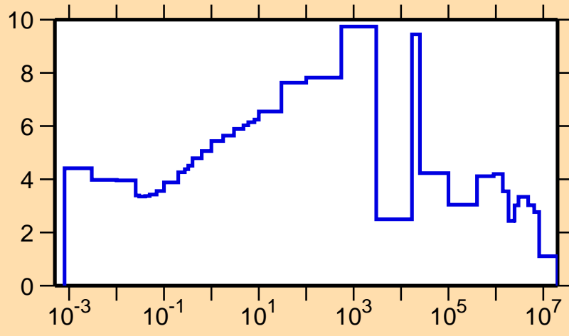
\Delta\sigma/\sigma vs. E for ^{203}\text{Tl}(n,\text{tot.})
