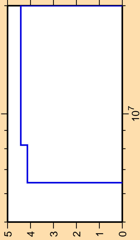
\Delta\sigma/\sigma vs. E for ^{203}\text{Tl}(n,n\text{cont.})
