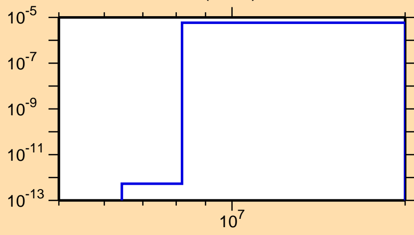
\sigma vs. E for ^{203}\text{Tl}(n,n\alpha)
