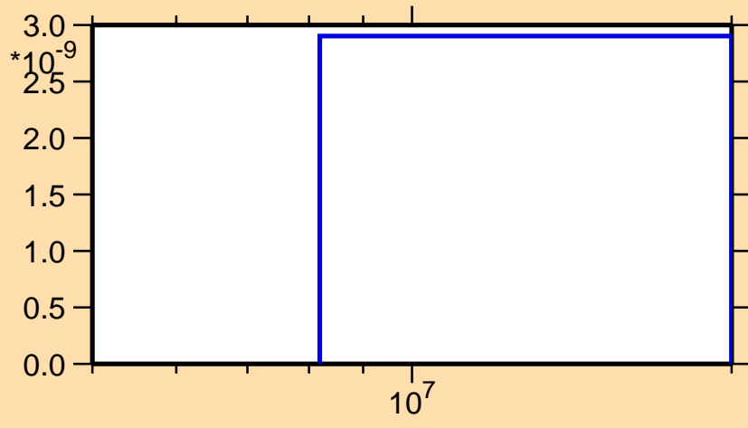
\sigma vs. E for ^{203}\text{Tl}(n,nd)
