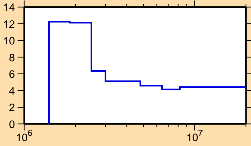
\Delta\sigma/\sigma vs. E for ^{203}\text{Tl}(n,ncont.)
