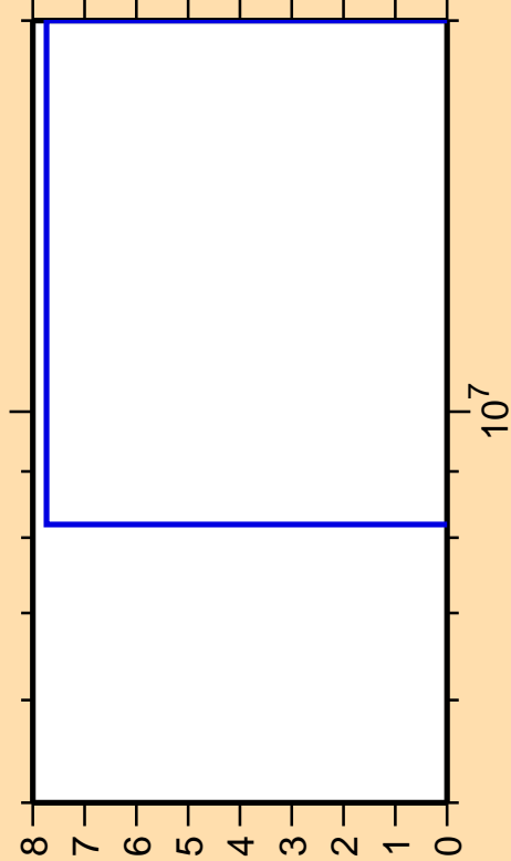
\Delta\sigma/\sigma vs. E for ^{203}\text{Tl}(n,3n)
