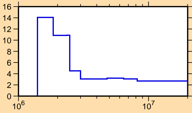
\Delta\sigma/\sigma vs. E for ^{203}\text{Tl}(n,n\text{onel.})
