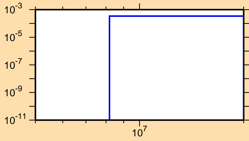
\sigma vs. E for ^{203}\text{Tl}(n,np)
