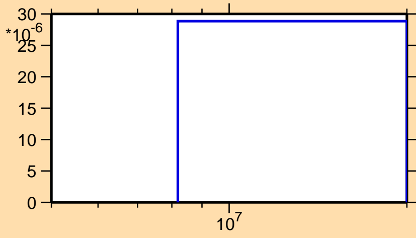
\sigma vs. E for ^{203}\text{Tl}(n,t)
