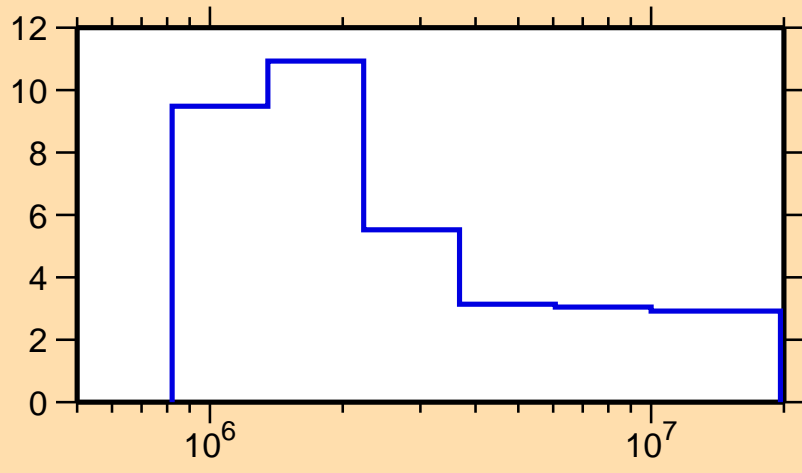
\Delta\sigma/\sigma vs. E for ^{204}\text{Tl}(n,n\text{onel.})
