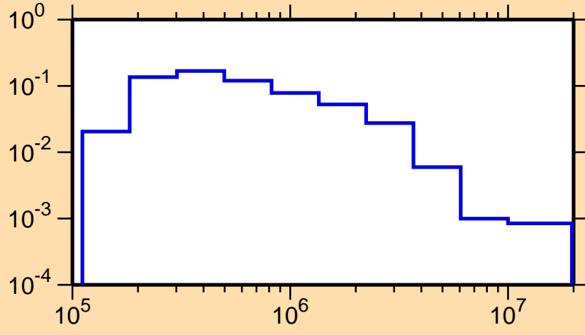
\sigma vs. E for ^{204}\text{Tl}(n,n_1)
