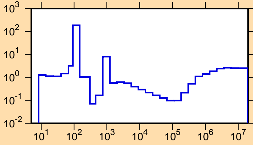
\sigma vs. E for ^{204}\text{Tl}(n,\text{nonel.})
