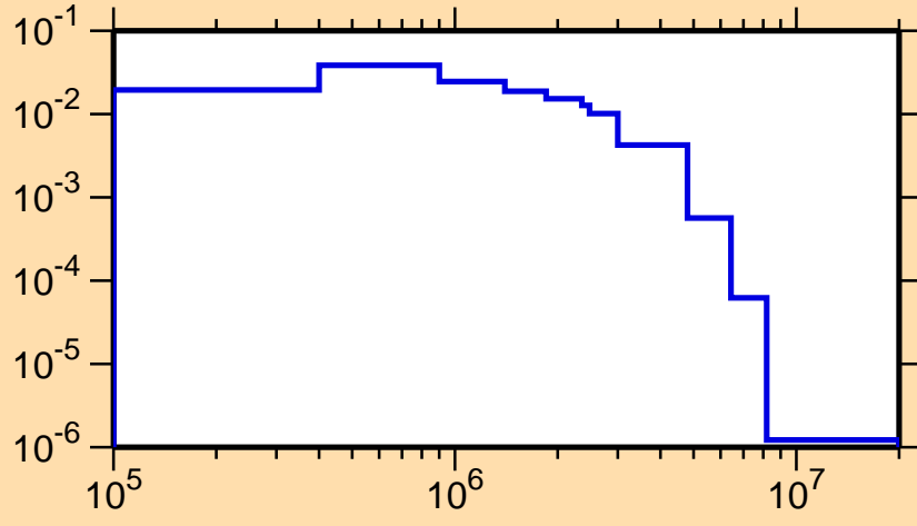
\sigma vs. E for ^{204}\text{Tl}(n,n_2)
