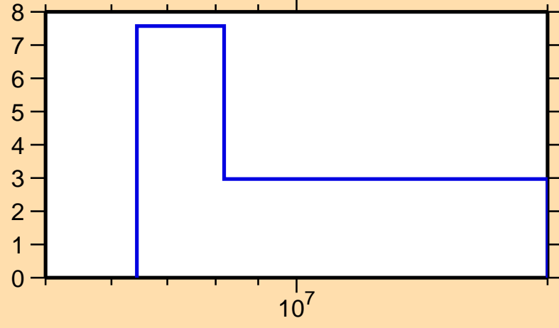
\Delta\sigma/\sigma vs. E for ^{204}\text{Tl}(n,2n)
