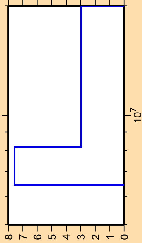
\Delta\sigma/\sigma vs. E for ^{204}\text{Tl}(n,2n)
