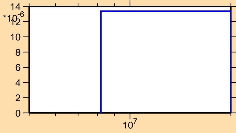
\sigma vs. E for ^{204}\text{Tl}(n,t)
