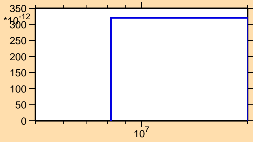
\sigma vs. E for ^{204}\text{Tl}(n,nt)
