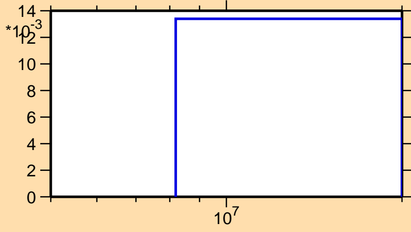
\sigma vs. E for ^{204}\text{Tl}(n,3n)
