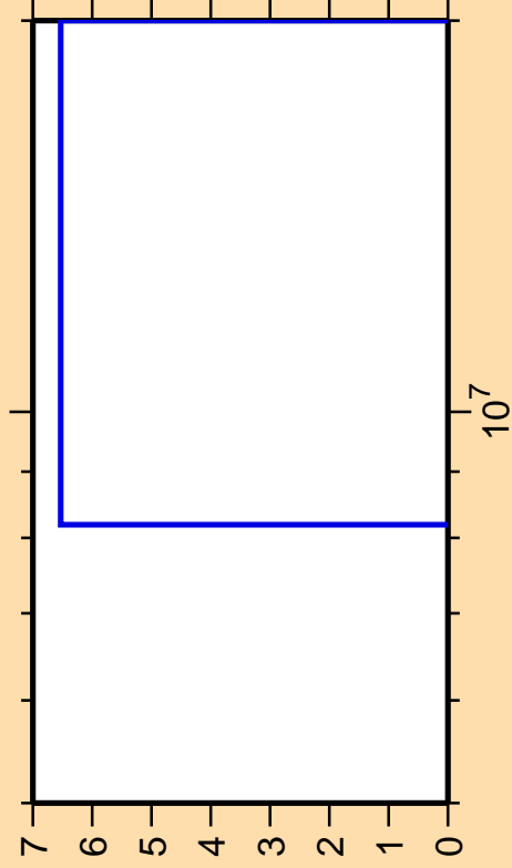
\Delta\sigma/\sigma vs. E for ^{204}\text{Tl}(n,3n)
