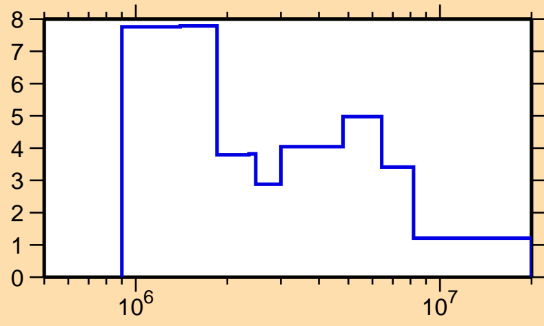
\Delta\sigma/\sigma vs. E for ^{204}\text{Tl}(n,el.)
