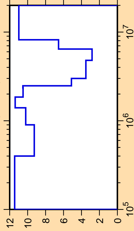
\Delta\sigma/\sigma vs. E for ^{204}\text{Tl}(n,\text{inel.})
