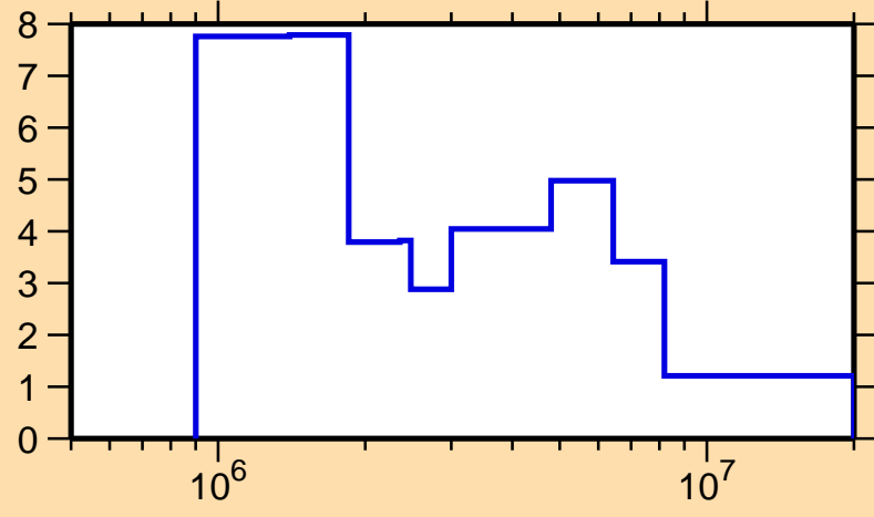
\Delta\sigma/\sigma vs. E for ^{204}\text{Tl}(n,\text{el.})
