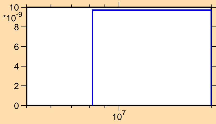
\sigma vs. E for ^{204}\text{Tl}(n,\text{nd})
