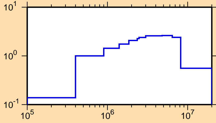
\sigma vs. E for ^{204}\text{Tl}(n,\text{inel.})
