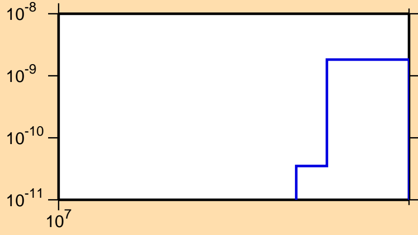
\sigma vs. E for ^{205}\text{Tl}(n,2n\alpha)
