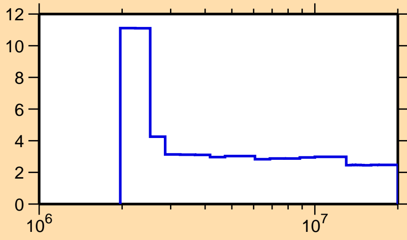
\Delta\sigma/\sigma vs. E for ^{205}\text{Tl}(n,n\text{onel.})
