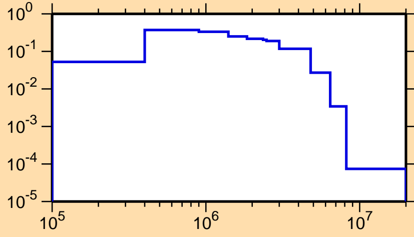
\sigma vs. E for ^{206}\text{Tl}(n,n_1)
