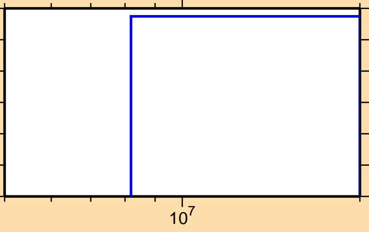
\sigma vs. E for ^{206}\text{Tl}(n,t)
