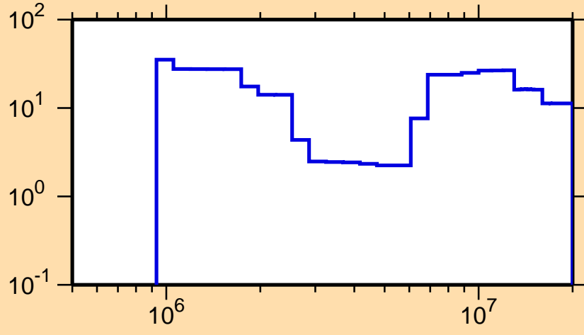
\Delta\sigma/\sigma vs. E for ^{206}\text{Tl}(n,ncont.)
