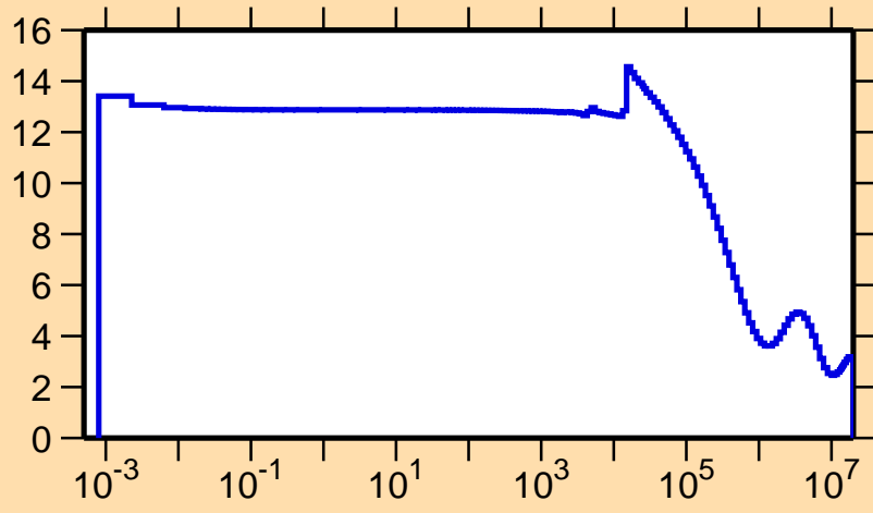
\sigma vs. E for ^{206}\text{Tl}(n,\text{el.})
