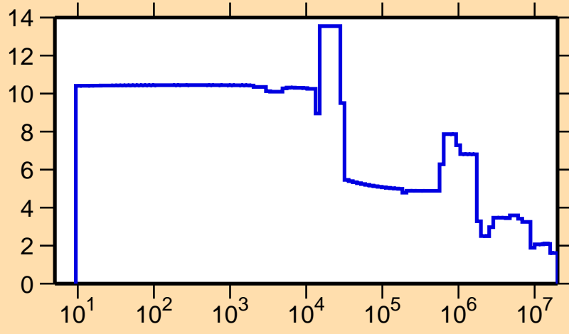
\Delta\sigma/\sigma vs. E for ^{206}\text{Tl}(n,\text{tot.})
