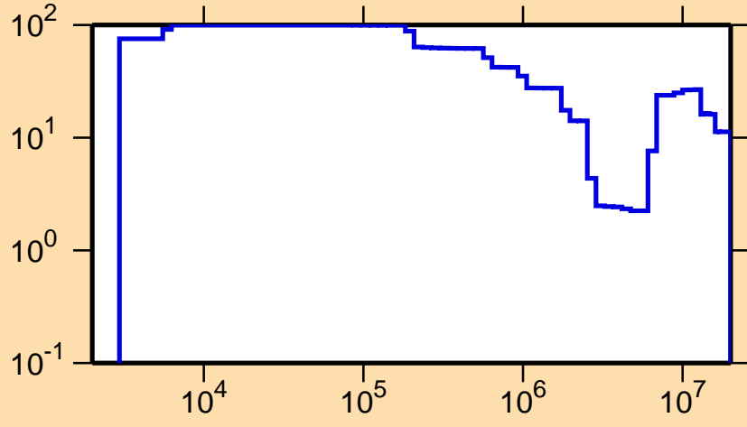
\Delta\sigma/\sigma vs. E for ^{206}\text{Tl}(n,n\text{cont.})
