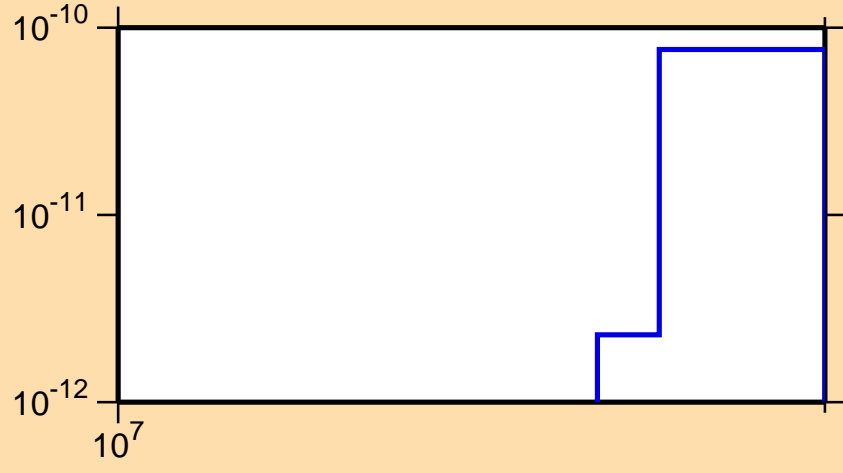
\sigma vs. E for ^{206}\text{Tl}(n,\text{He}3)
