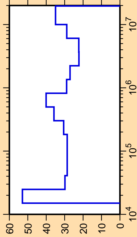
\Delta\sigma/\sigma vs. E for ^{206}\text{Tl}(n,n_4)
