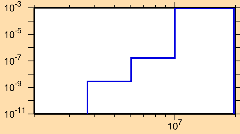
\sigma vs. E for ^{206}\text{Tl}(n,p)
