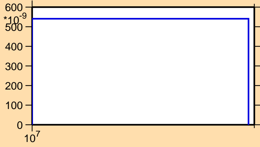
\sigma vs. E for ^{206}\text{Tl}(n,2n\alpha)
