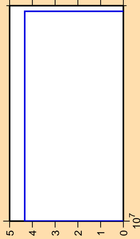
\Delta\sigma/\sigma vs. E for ^{206}\text{Tl}(n,\text{He}3)
