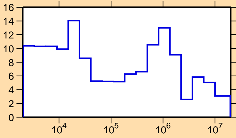
\Delta\sigma/\sigma vs. E for ^{206}\text{Tl}(n, el.)
