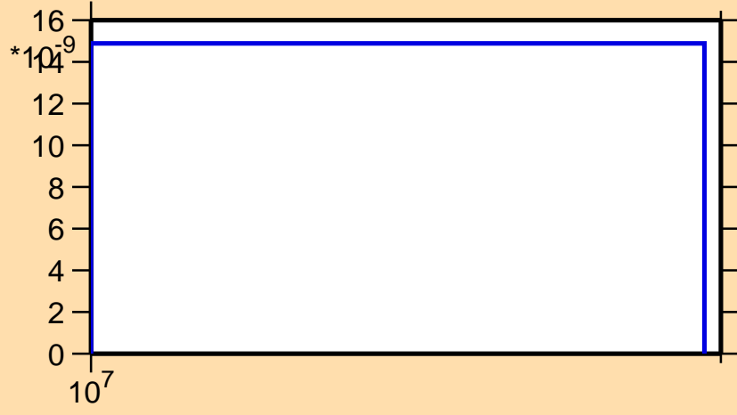
\sigma vs. E for ^{206}\text{Tl}(n,2np)
