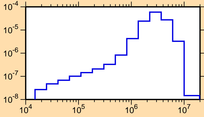
\sigma vs. E for ^{206}\text{Tl}(n,n_4)
