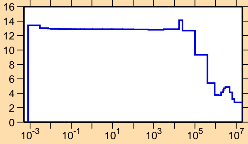
\sigma vs. E for ^{206}\text{Tl}(n,\text{el.})
