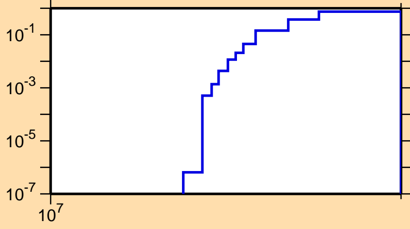
\sigma vs. E for ^{207}\text{Tl}(n,3n)
