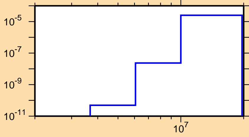
\sigma vs. E for ^{207}\text{Tl}(n,\alpha)
