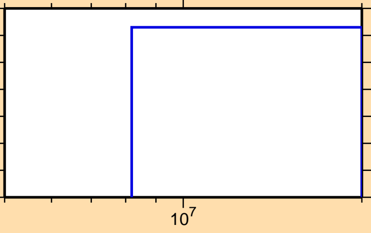
\sigma vs. E for ^{207}\text{Tl}(n,np)
