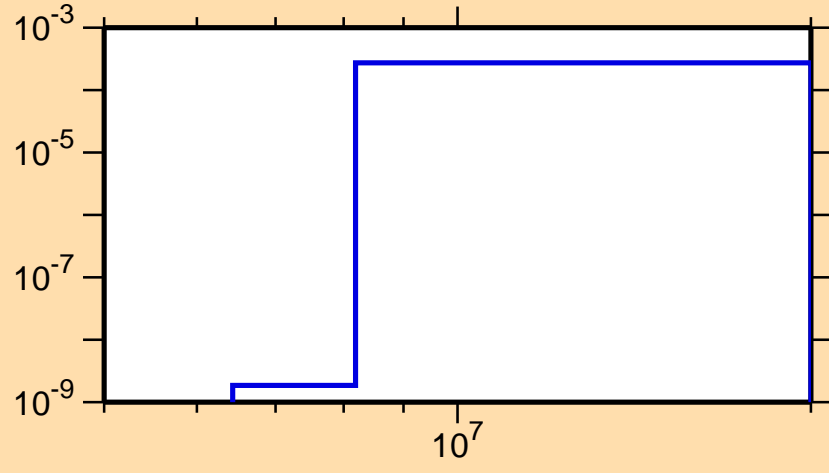
\sigma vs. E for ^{207}\text{Tl}(n,p)
