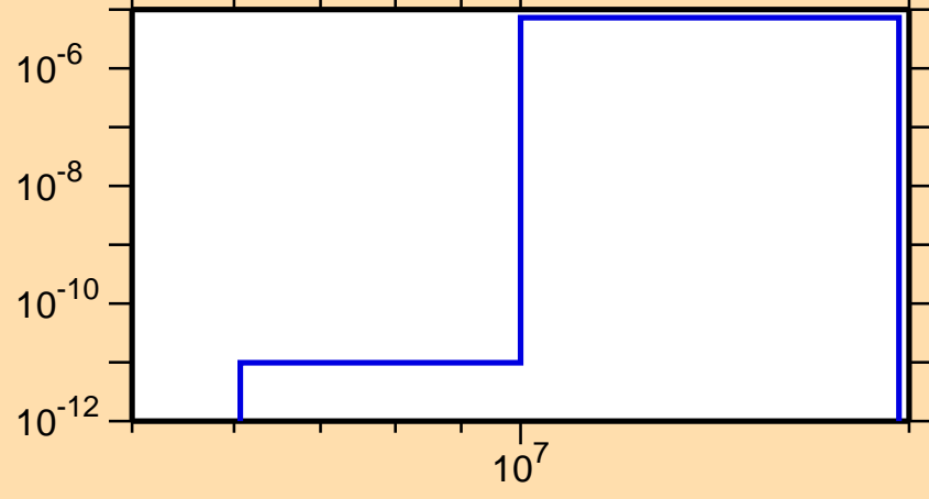
\sigma vs. E for ^{207}\text{Tl}(n,d)
