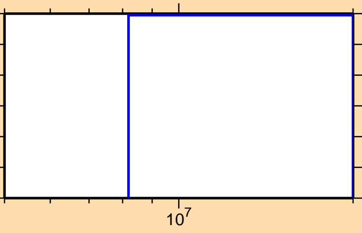
\sigma vs. E for ^{207}\text{Tl}(n,nt)
