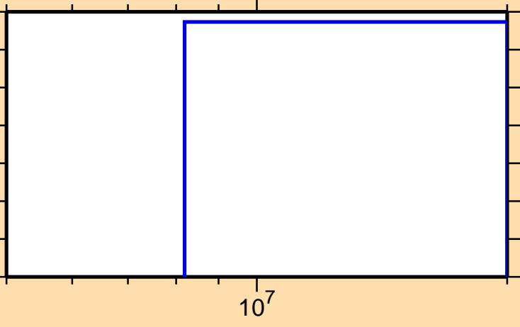
\sigma vs. E for ^{208}\text{Tl}(n,nt)
