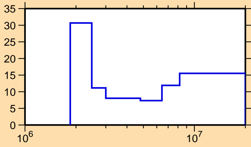
\Delta\sigma/\sigma vs. E for ^{208}\text{Tl}(n,n\text{cont.})
