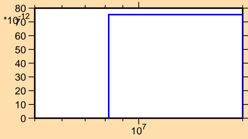
\sigma vs. E for ^{208}\text{Tl}(n,2n\alpha)
