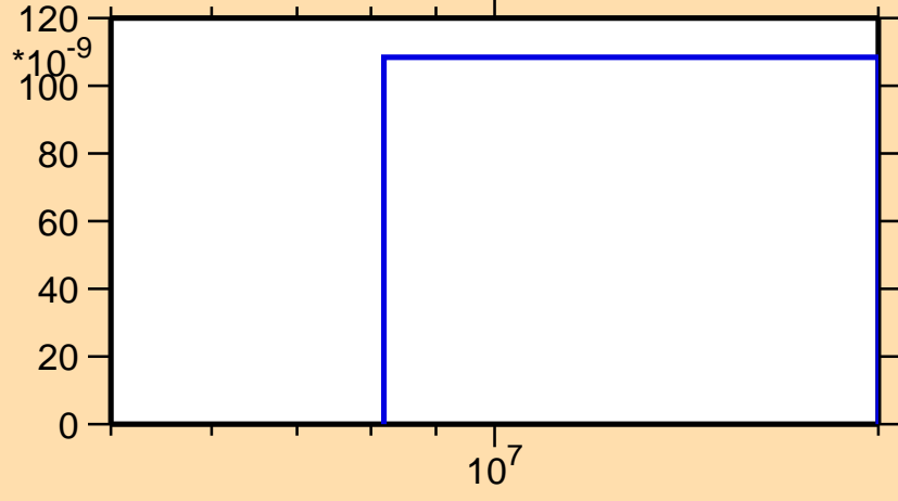
\sigma vs. E for ^{208}\text{Tl}(n,nd)
