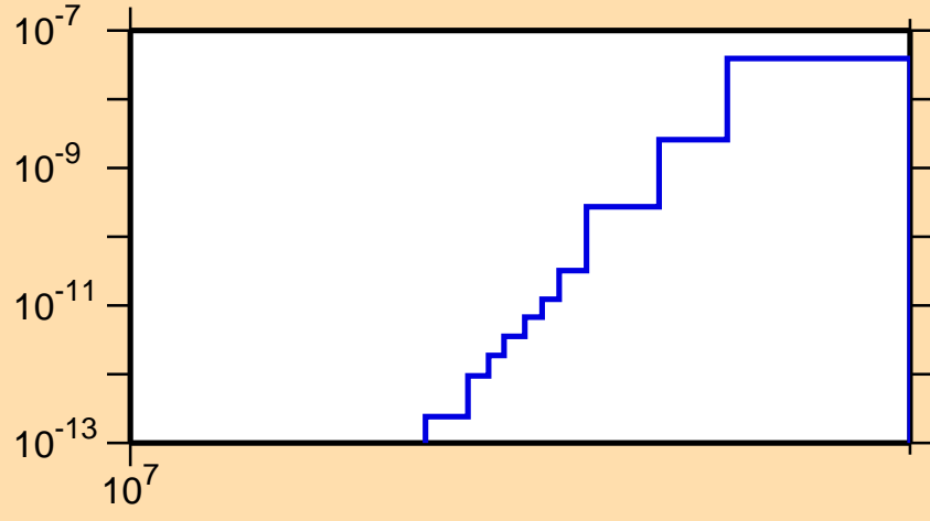
\sigma vs. E for ^{209}\text{Tl}(n,2n\alpha)
