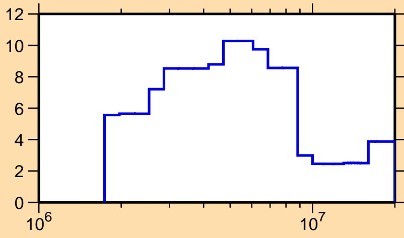
\Delta\sigma/\sigma vs. E for ^{209}\text{Tl}(n, el.)
