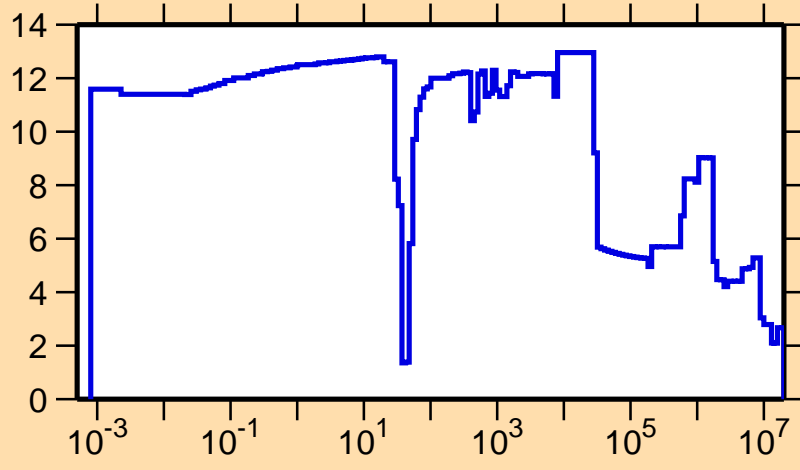
\Delta\sigma/\sigma vs. E for ^{209}\text{Tl}(n,\text{tot.})
