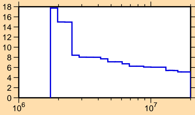
\Delta\sigma/\sigma vs. E for ^{209}\text{Tl}(n, \text{nonel.})
