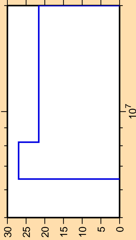
\Delta\sigma/\sigma vs. E for ^{209}\text{Tl}(n,p)
