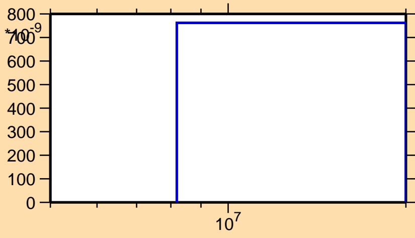
\sigma vs. E for ^{209}\text{Tl}(n,nt)
