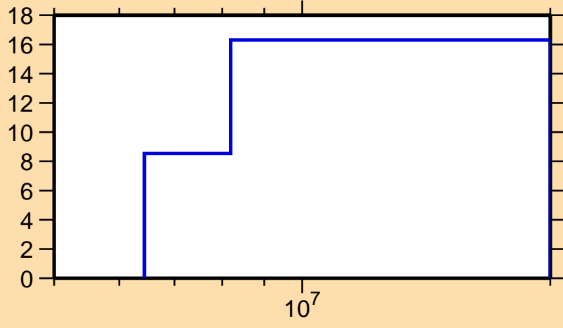
\Delta\sigma/\sigma vs. E for ^{209}\text{Tl}(n,ncont.)
