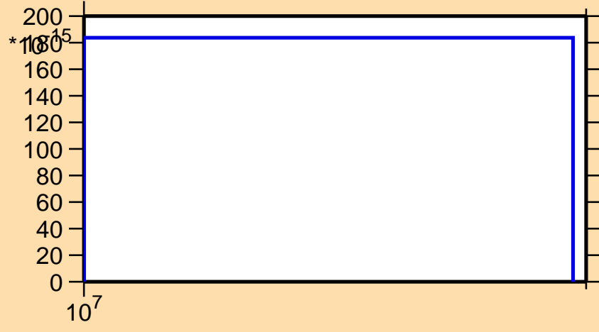
\sigma vs. E for ^{210}\text{Tl}(\text{mt } 11)
