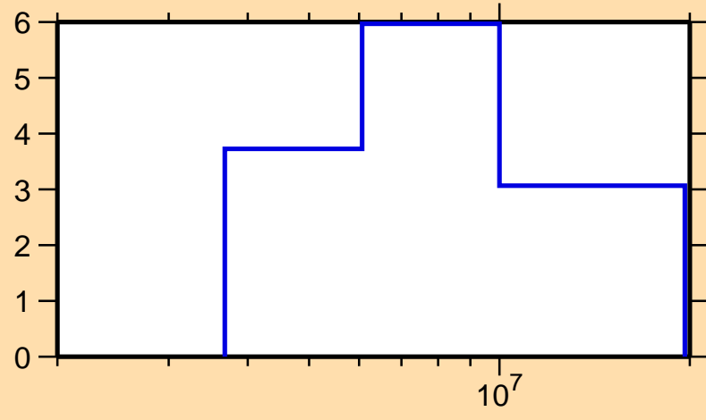
\Delta\sigma/\sigma vs. E for ^{210}\text{Tl}(n,\text{tot.})
