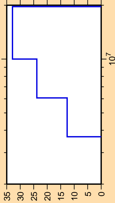
\Delta\sigma/\sigma vs. E for ^{210}\text{Tl}(n,n\text{cont.})
