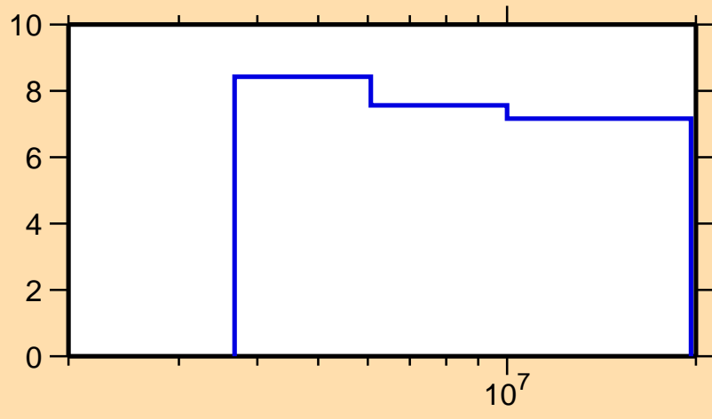
\Delta\sigma/\sigma vs. E for ^{210}\text{Tl}(n,\text{nonel.})
