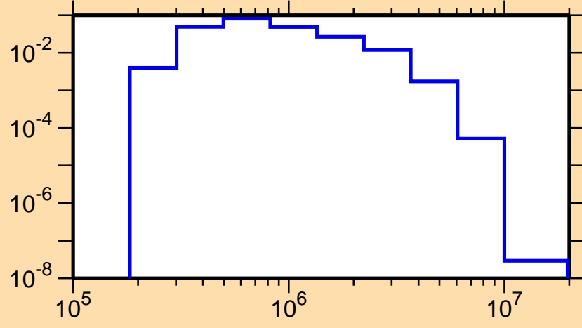
\sigma vs. E for ^{210}\text{Tl}(n,n_2)
