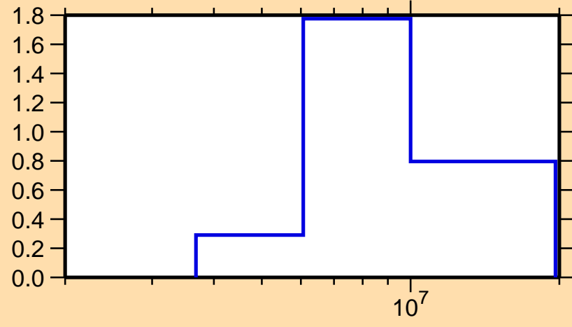
\sigma vs. E for ^{210}\text{Tl}(n,2n)
