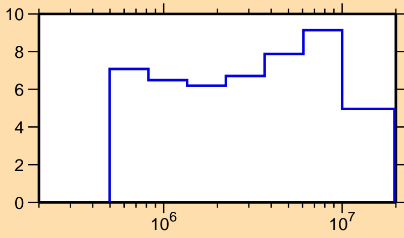
\Delta\sigma/\sigma vs. E for ^{210}\text{Tl}(n, el.)
