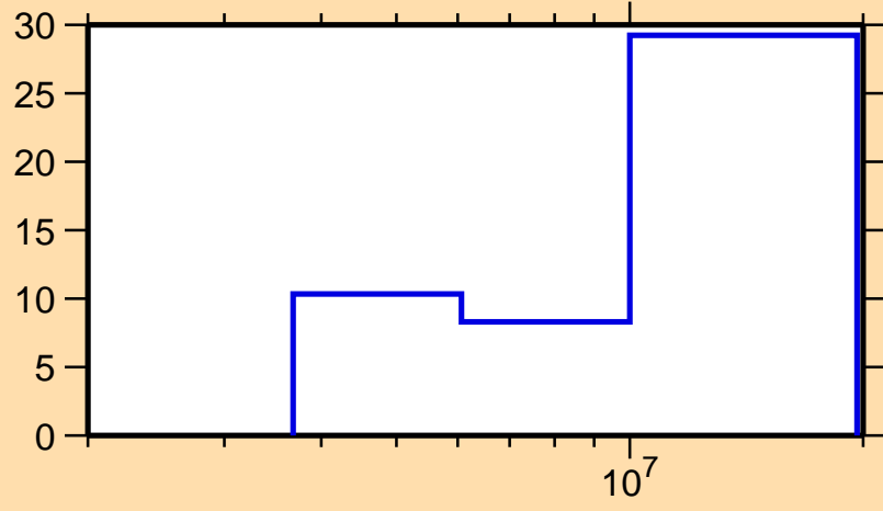
\Delta\sigma/\sigma vs. E for ^{210}\text{Tl}(n,2n)
