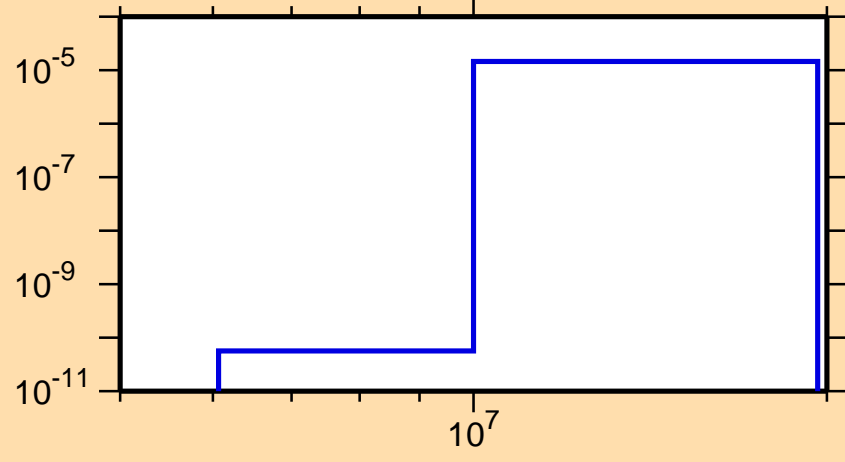
\sigma vs. E for ^{210}\text{Tl}(n,n\alpha)
