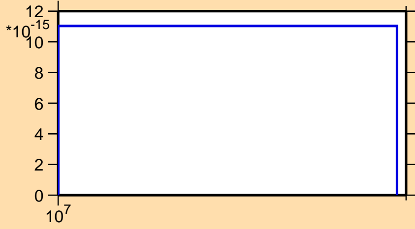
\sigma vs. E for ^{210}\text{Tl}(n,3n\alpha)
