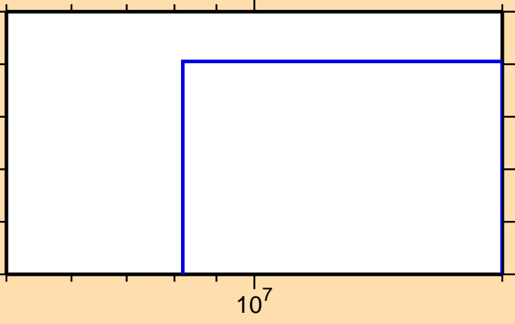
\sigma vs. E for ^{210}\text{Tl}(n,2np)
