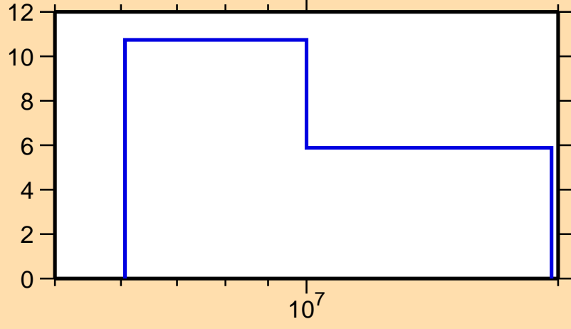
\Delta\sigma/\sigma vs. E for ^{211}\text{Tl}(n,el.)
