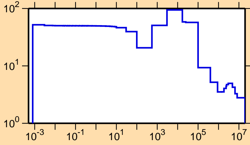
\sigma vs. E for ^{211}\text{Tl}(n,\text{el.})
