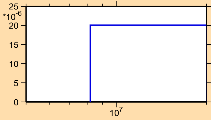
\sigma vs. E for ^{211}\text{Tl}(n,t)
