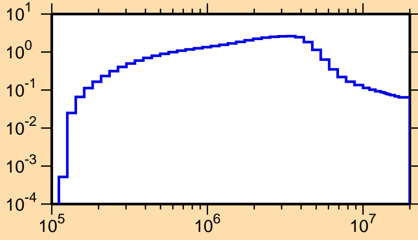
\sigma vs. E for ^{212}\text{Tl}(n,n\text{cont.})
