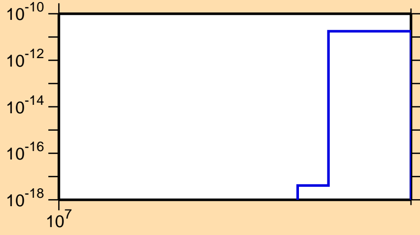
\sigma vs. E for ^{212}\text{Tl} (mt 11)
