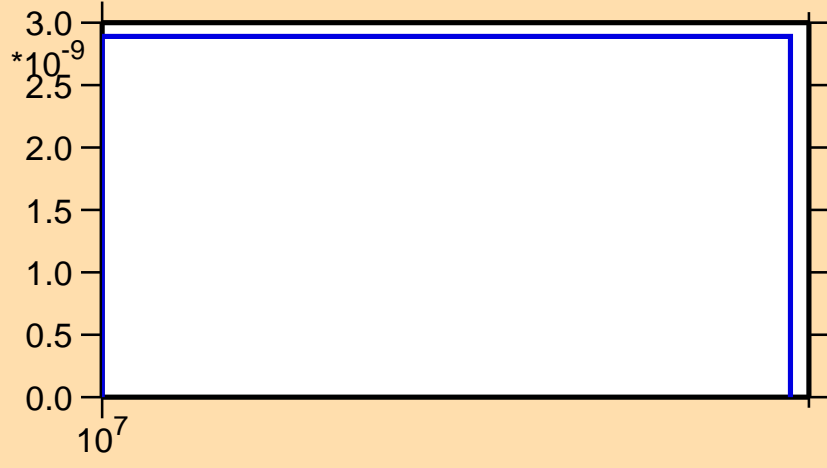
\sigma vs. E for ^{212}\text{Tl}(n,2np)
