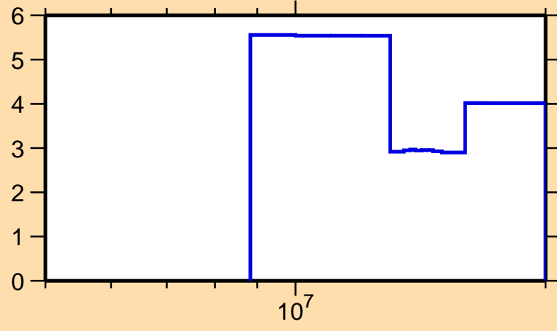
\Delta\sigma/\sigma vs. E for ^{213}\text{Tl}(n,\text{tot.})
