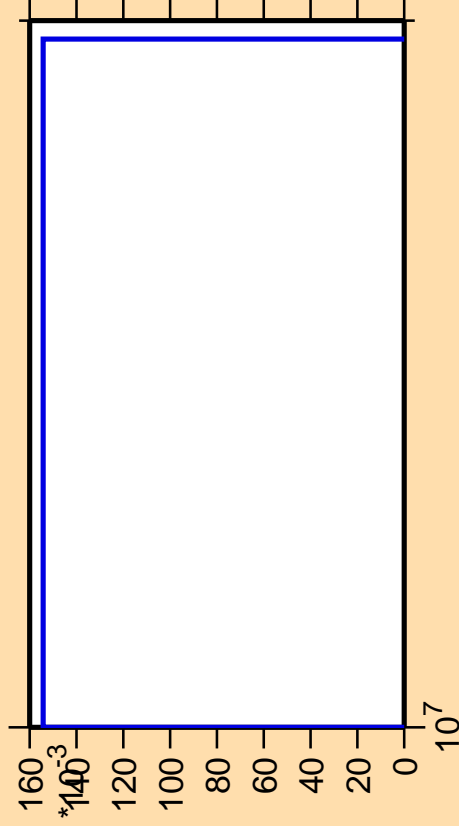
\Delta\sigma/\sigma vs. E for ^{213}\text{Tl} (mt 11)
