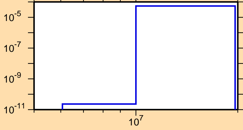
\sigma vs. E for ^{213}\text{Tl}(n,p)
