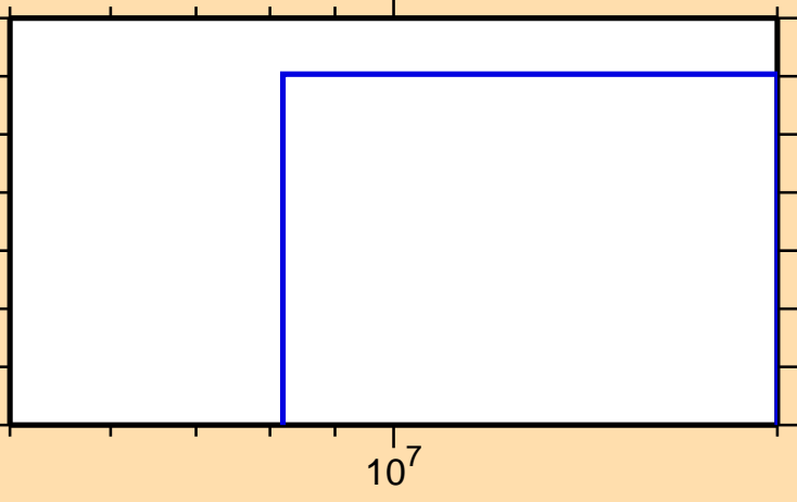
\sigma vs. E for ^{213}\text{Tl}(n,t)
