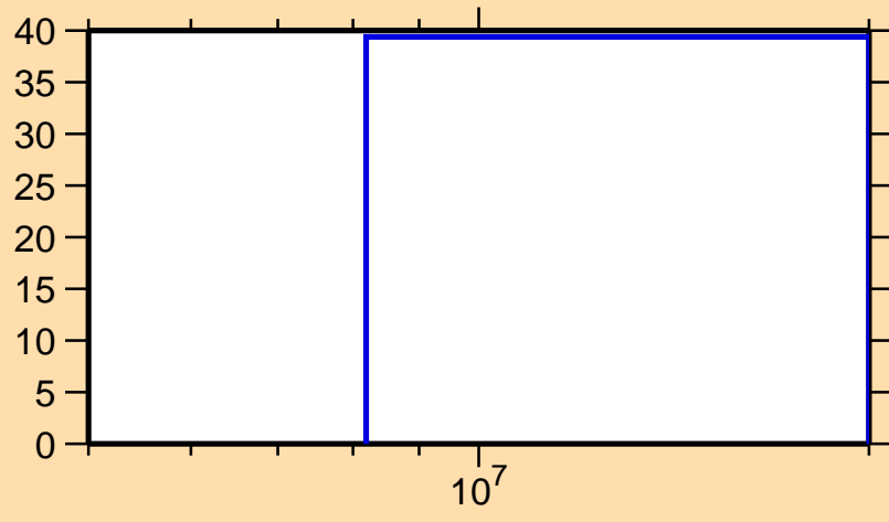
\Delta\sigma/\sigma vs. E for ^{213}\text{Tl}(n,ncont.)
